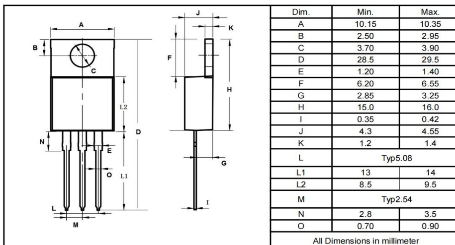
TO-220F
